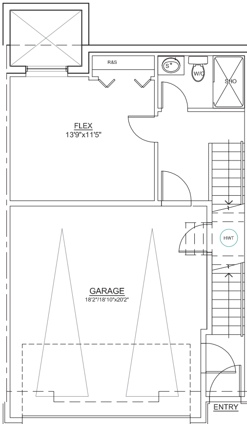
PLAN C - LOWER FLOOR PLAN (FIN. AREA 415 s.f.) (UNFIN. AREA 390 s.f.)
