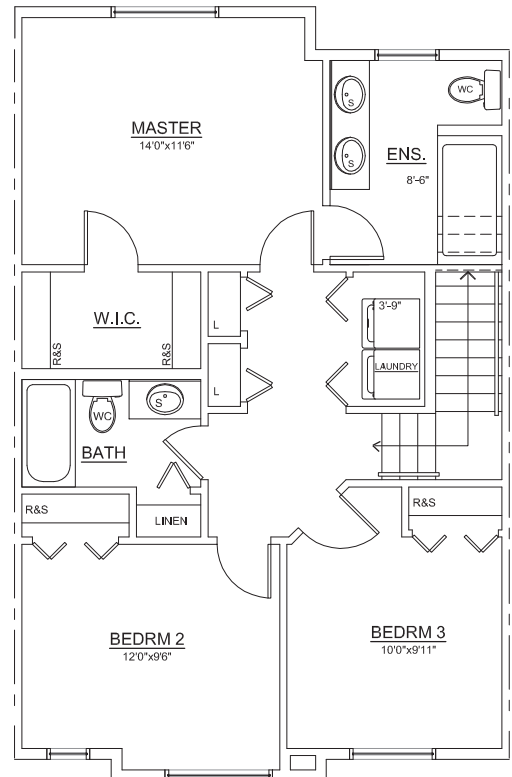
PLAN C - UPPER FLOOR PLAN (797 s.f.)
