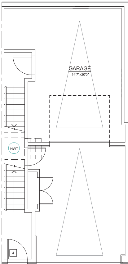
PLAN B1 - LOWER FLOOR PLAN (FIN. AREA 139 s.f.) (UNFIN. AREA 347 s.f.)
