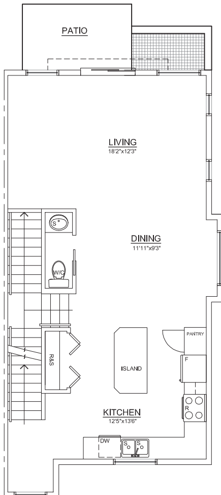
PLAN B1 - MAIN FLOOR PLAN (707 s.f.)
