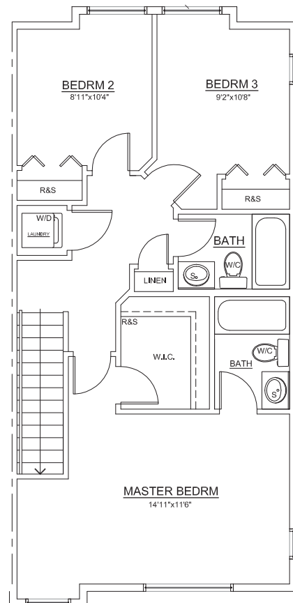
PLAN B1 - UPPER FLOOR PLAN (738 s.f.)
