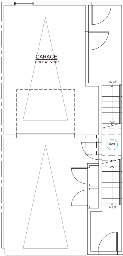
PLAN B - LOWER FLOOR PLAN (FIN. AREA 192 s.f.) (UNFIN. AREA 290 s.f.)
