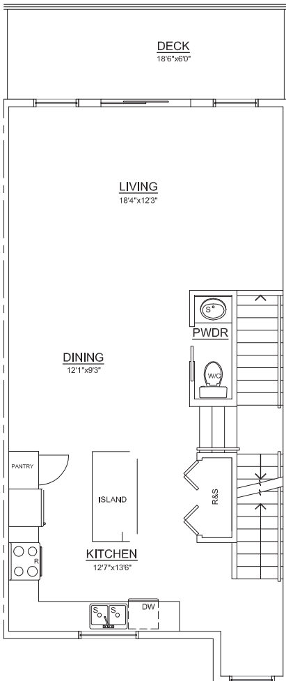
PLAN B - MAIN FLOOR PLAN (699 s.f.)
