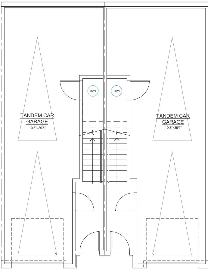
PLAN D - LOWER FLR PLAN (FIN AREA 121 s.f.) (UNFIN AREA 526 s.f.)
