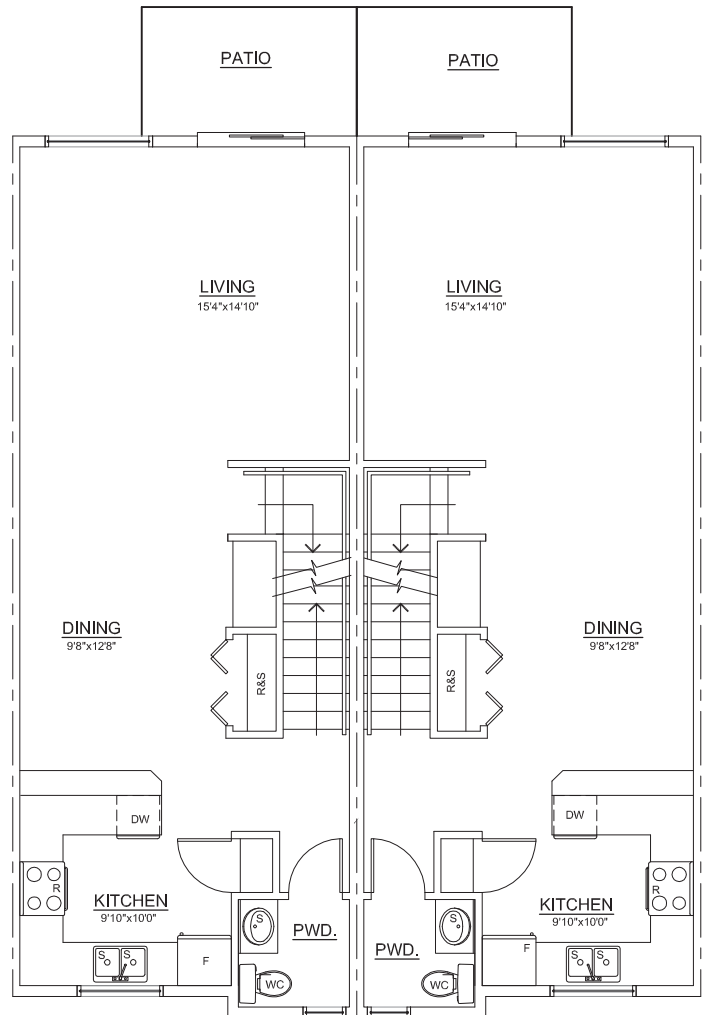
PLAN D - MAIN FLR PLAN (646 s.f.)
