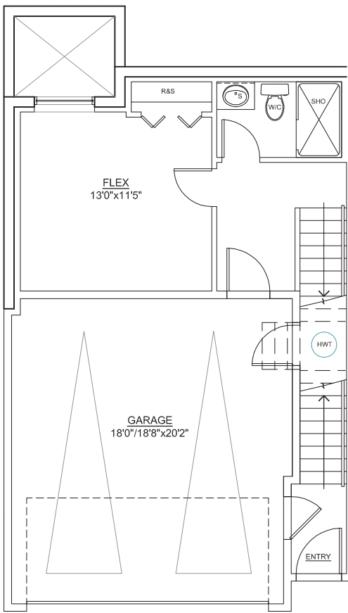
PLAN C1 - LOWER FLOOR PLAN (FIN. AREA 415 s.f.) (UNFIN. AREA 390 s.f.)
