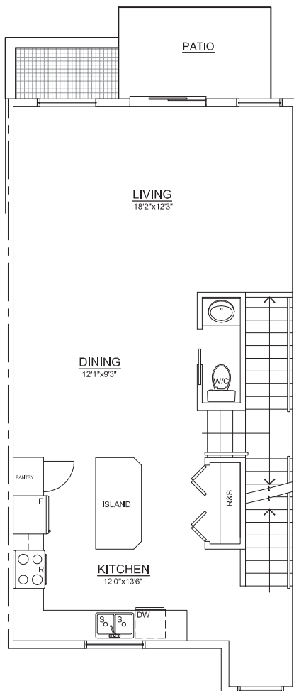
PLAN B2 - MAIN FLOOR PLAN (700 s.f.)
