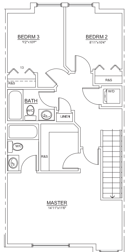
PLAN B2 - UPPER FLOOR PLAN (740 s.f.)
