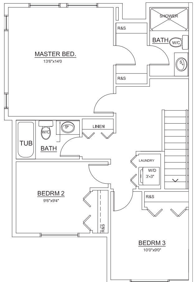
PLAN A - UPPER FLOOR PLAN (765 s.f.)
